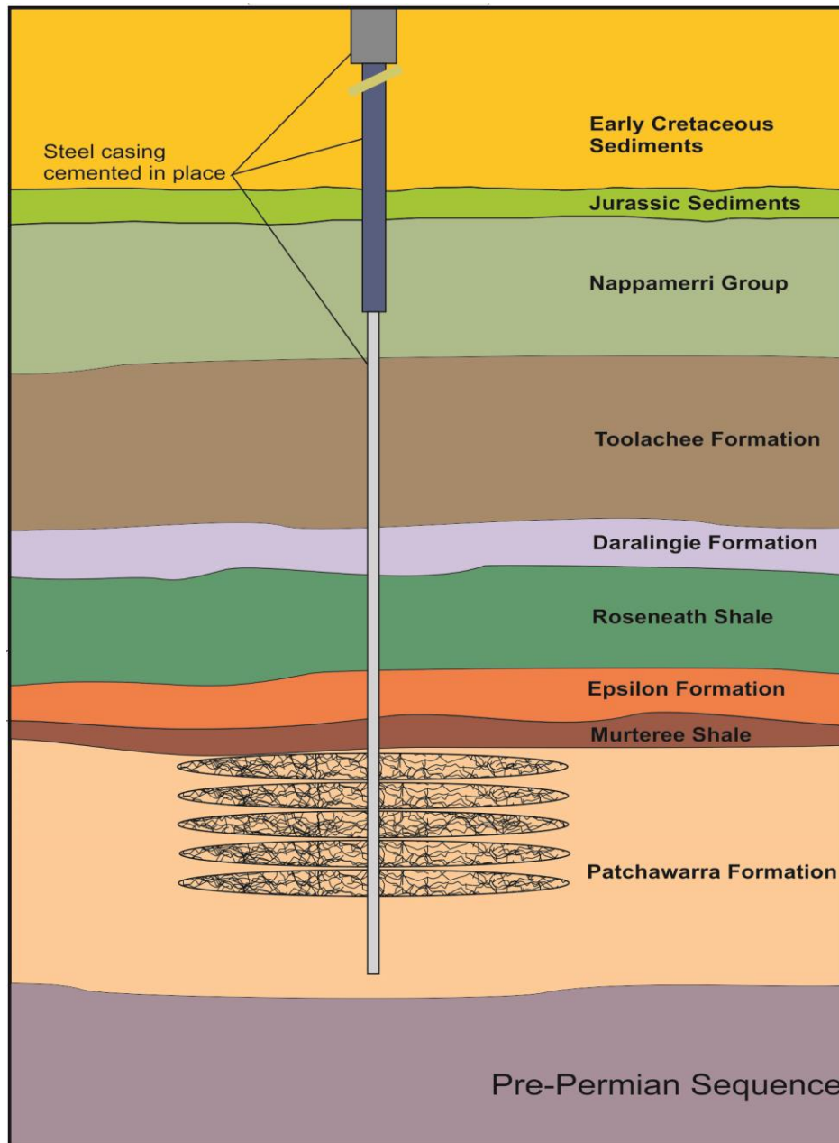
Diagram showing the Upper Patchawarra Stimulation zones in Hervey-1
